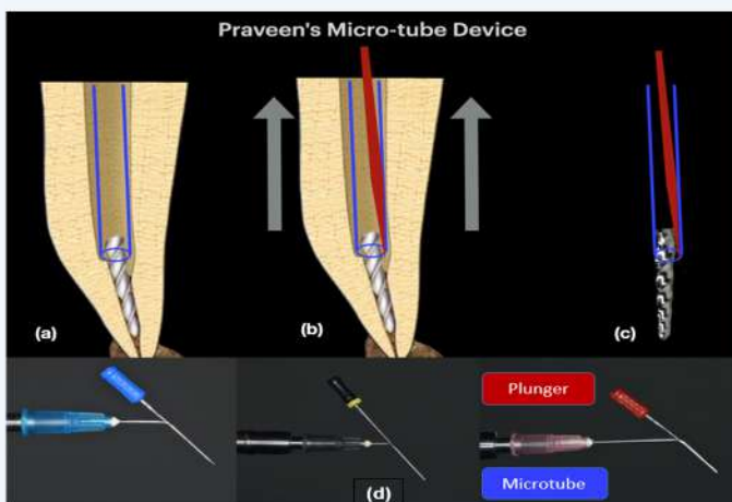
Figure 1: (a) The correct Microtube size is determined and inserted into the canal till the head of the file, till the head engulfs and is adapted around the broken fragment. (b) The plunger is then inserted to grip the broken file against the tube and (c) the entire assembly is pulled out with the broken file. (d) Three different sizes of Microtube and Plunger assembly are depicted.
